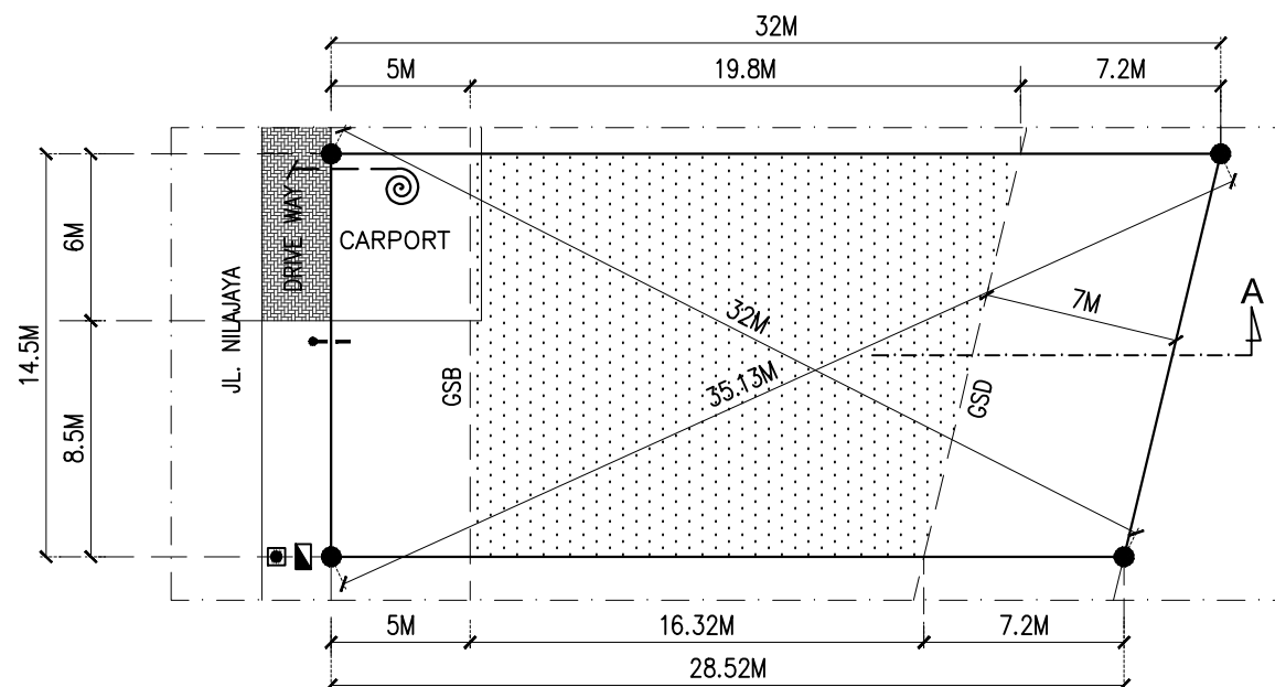
DENAH KAVLING JL. NILAJAYA NO. 37 SKALA 1 : 300
